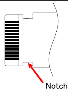
FFC/FPC temporary holding mechanism
