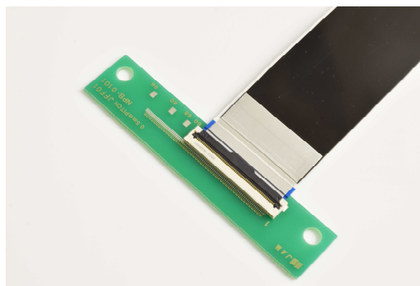
FFC/FPC temporary holding mechanism
